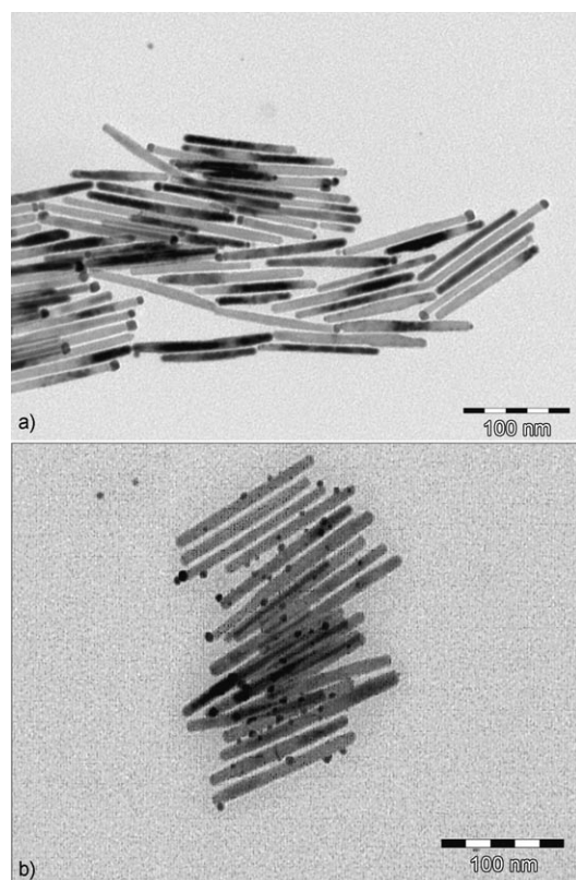
Figure 2. TEM images of a) gold-tipped Co nanorods prepared at 40°C and b) gold-decorated Co nanorods prepared at 20°C. For both, [\text{Co}] = 1.3 \times 10^{-3} \text{ M} , [\text{Au}] = 1.34 \times 10^{-4} \text{ M} , reaction time 48 h.
